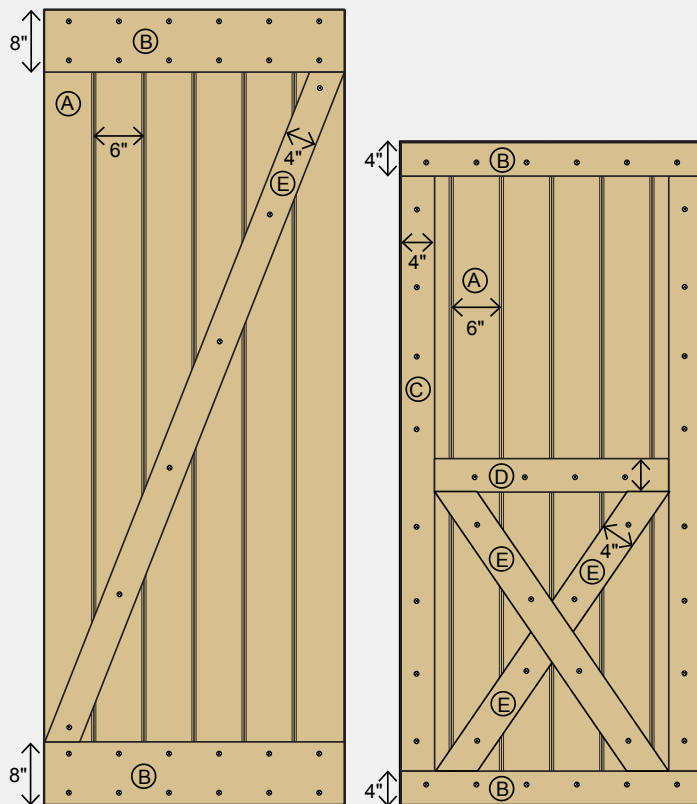
PLANK DOOR Shown here with 8'0" tall Z Barn Door
