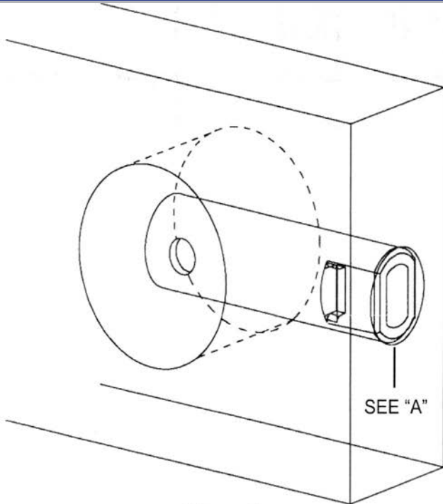
Figure 1 Typical 1-3/4" Exterior Door
