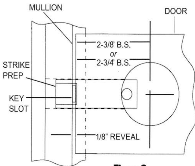
Figure 3 Front View
