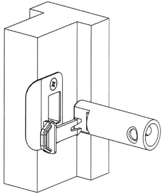
Figure 2 Typical Mullion or Astragal With Strike Plate Applied
