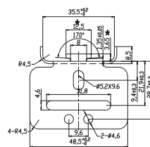
1000-R-BRKT Downward rear mounting bracket
