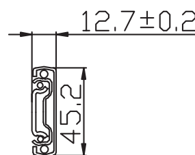
Optional Plastic Rear Socket
